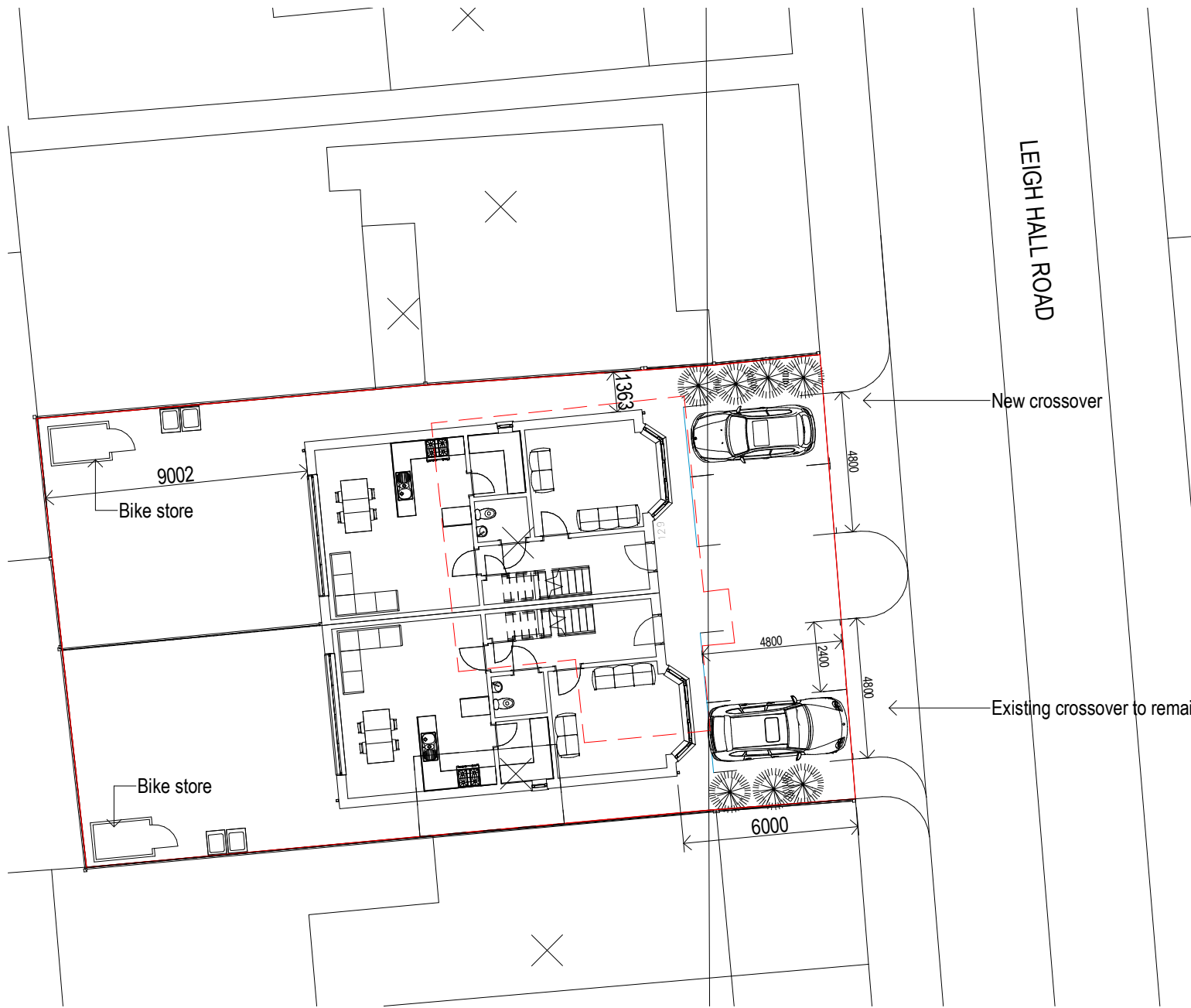
1 Site Plan - Proposed 1 : 200
